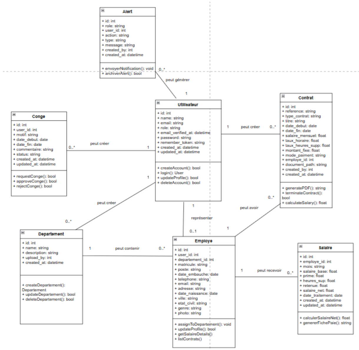
FIGURE 2.4 – Diagramme de classes
